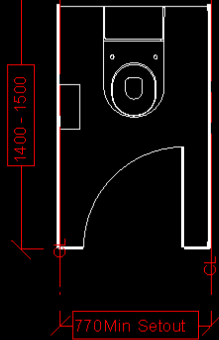
TOILET SET OUT
